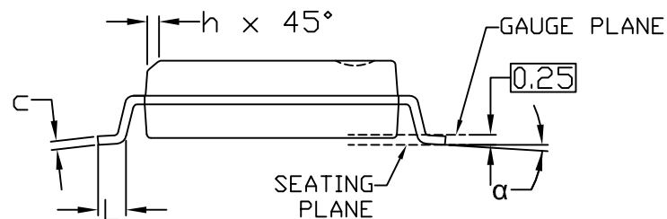
END VIEW
