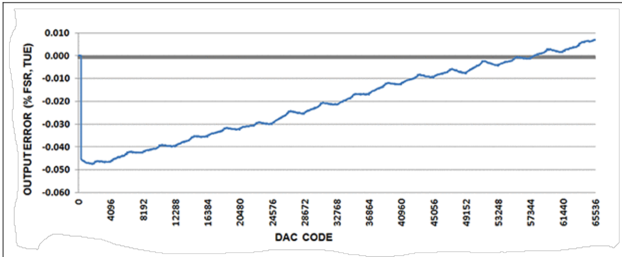
Figure 5. Output error for -10V to +10V output range, with 20% overrange.
