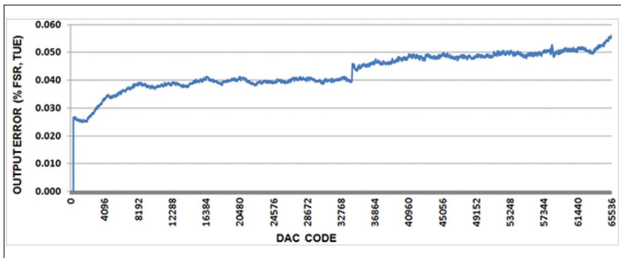
Figure 14. Output error for 0 to 20mA output range, with 20% overrange.
