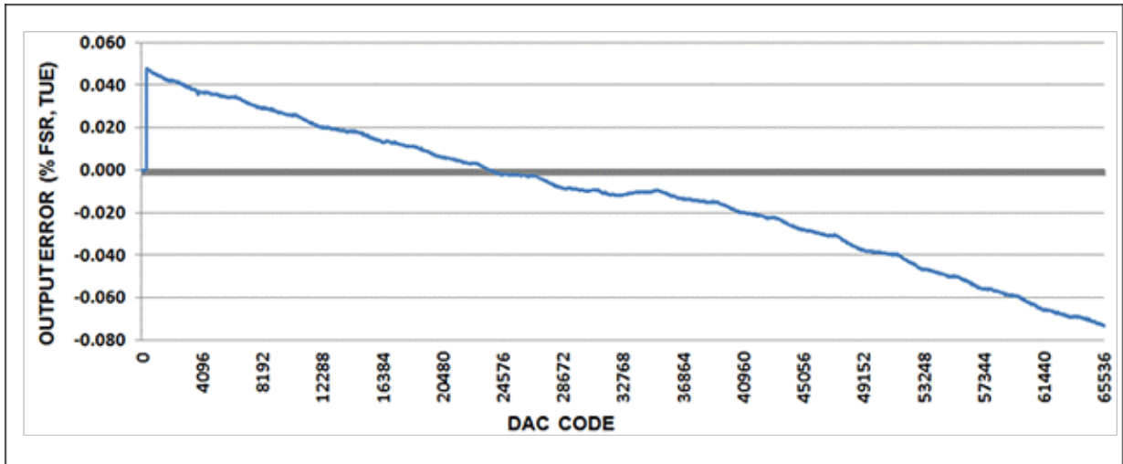
Figure 11. Output error for -20mA to +20mA output range, with 20% overrange.
