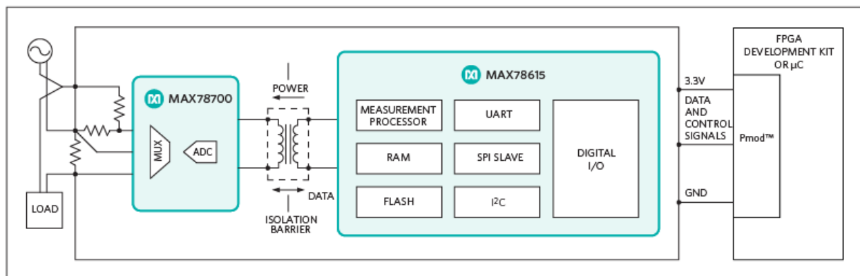
Figure 1. The Sonoma subsystem design block diagram.
