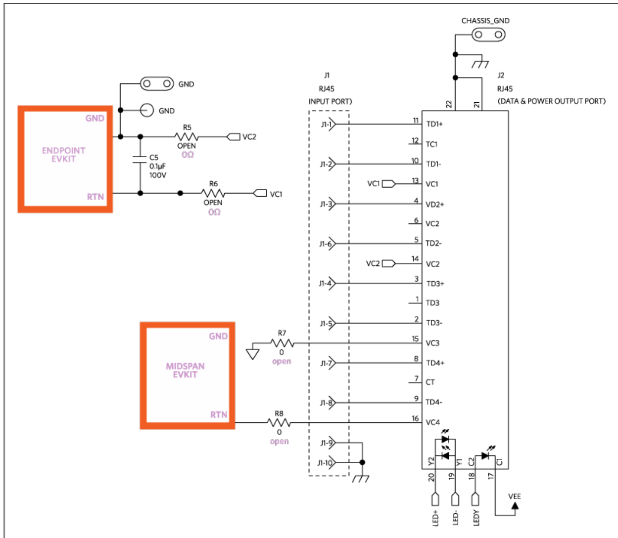
Figure 2. MAX5971A EV Kit modifications for a 2 x 2 Ethernet pair.
