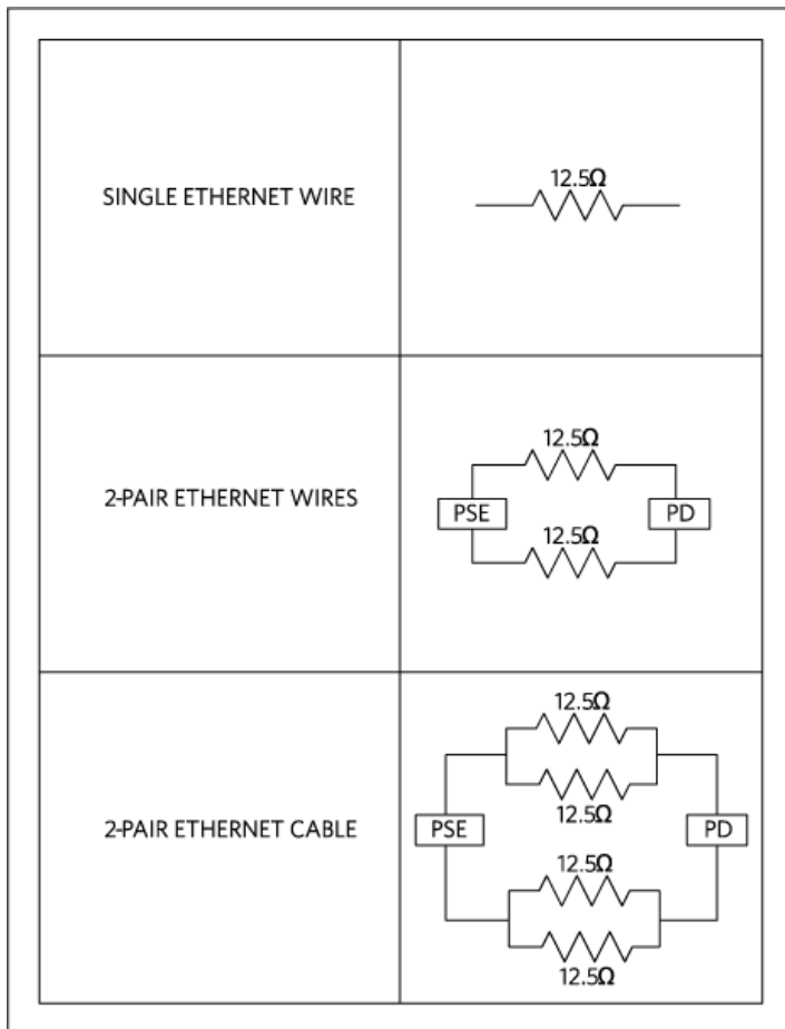
Figure 1. A 2 x 2 pair Ethernet cabling configuration.
