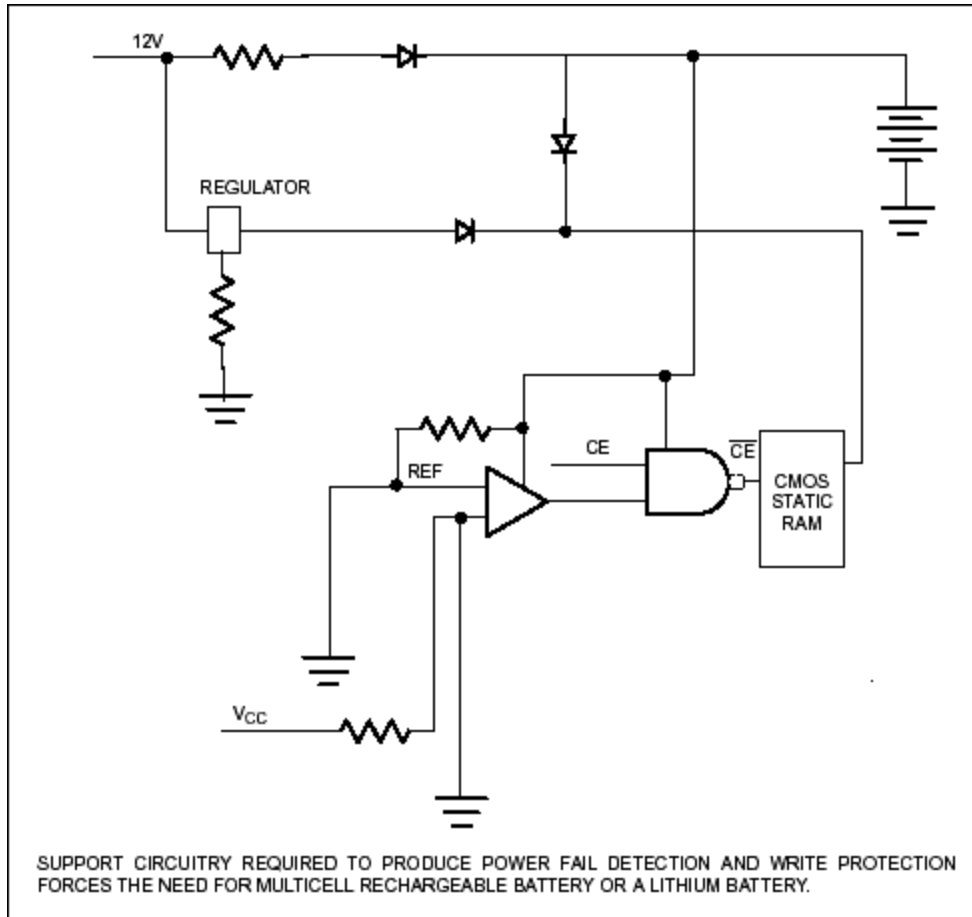
Figure 3. Power supply and battery isolation circuitry.
