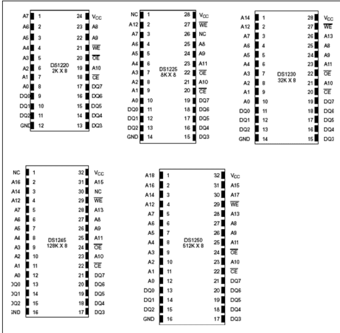
Figure 8. Dallas Semiconductor battery backup SRAM modules.
