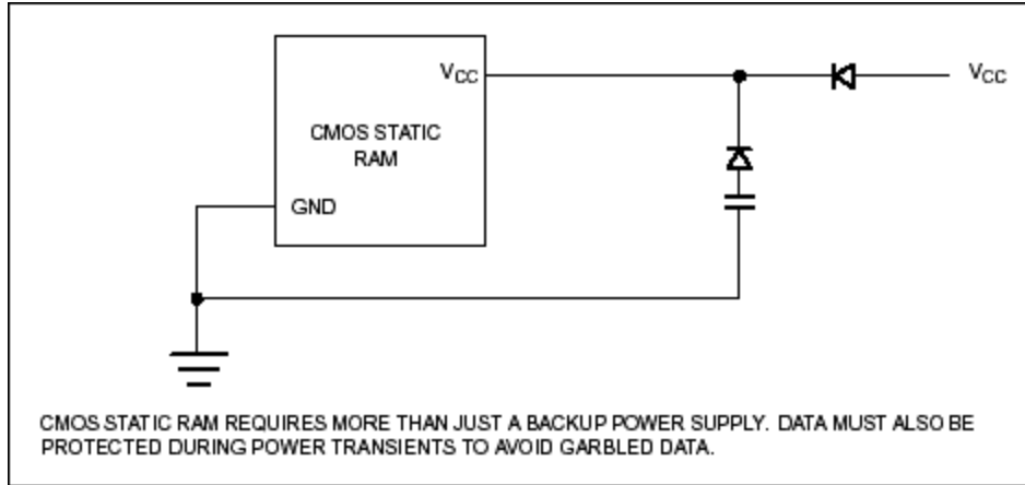
Figure 2. Battery backup circuit.
