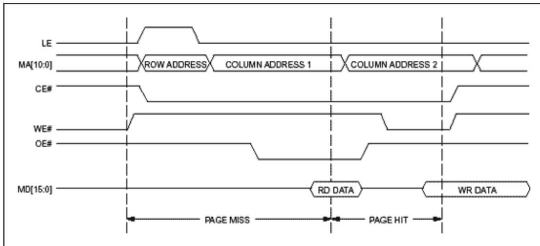
Figure 4. Portable applications: Intel 386SL CPU/NV SRAM timing.
