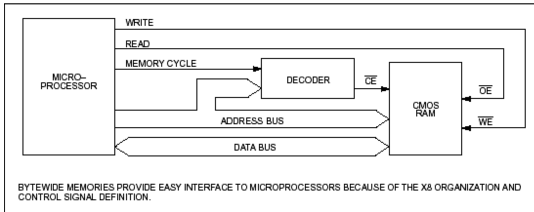
Figure 1. Byte-wide RAM to microprocessor interface.
