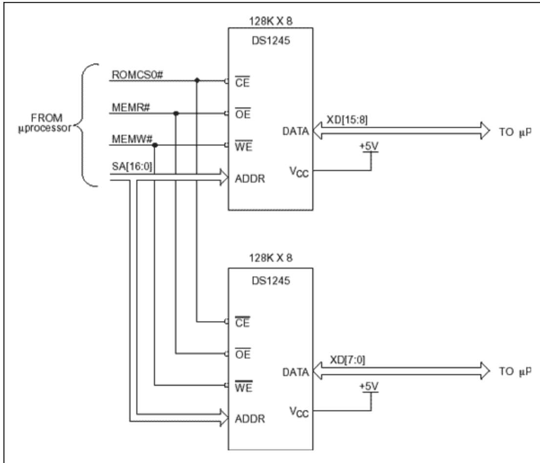
Figure 6. 16-Bit single-bank NV SRAM BIOS circuit.
