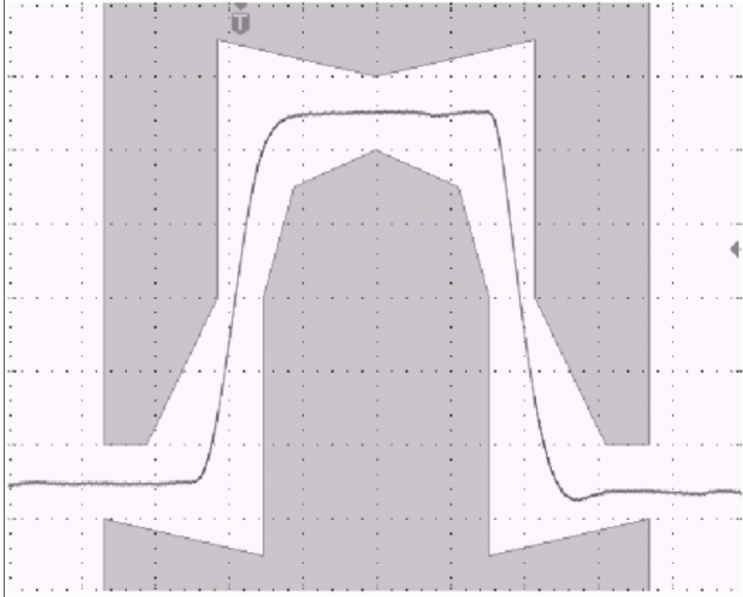
Figure 4. E3 Pulse (34.368 Mb/s).
