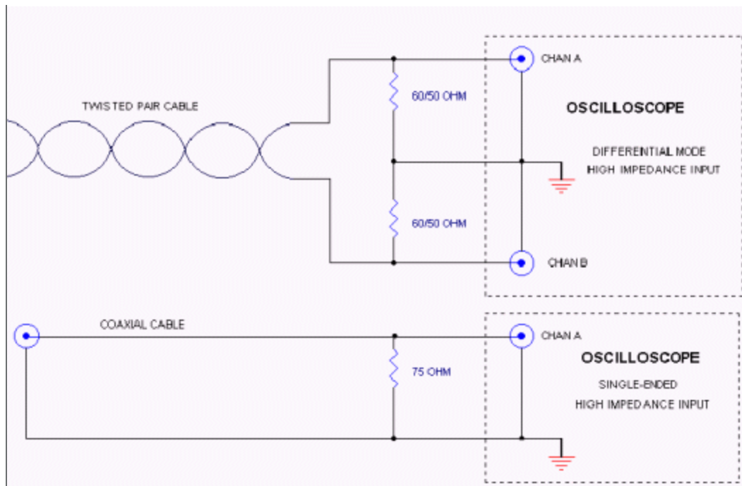
Figure 5. Line termination.
