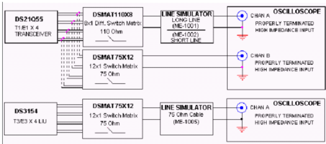
Figure 6. Pulse mask testing block diagram.
