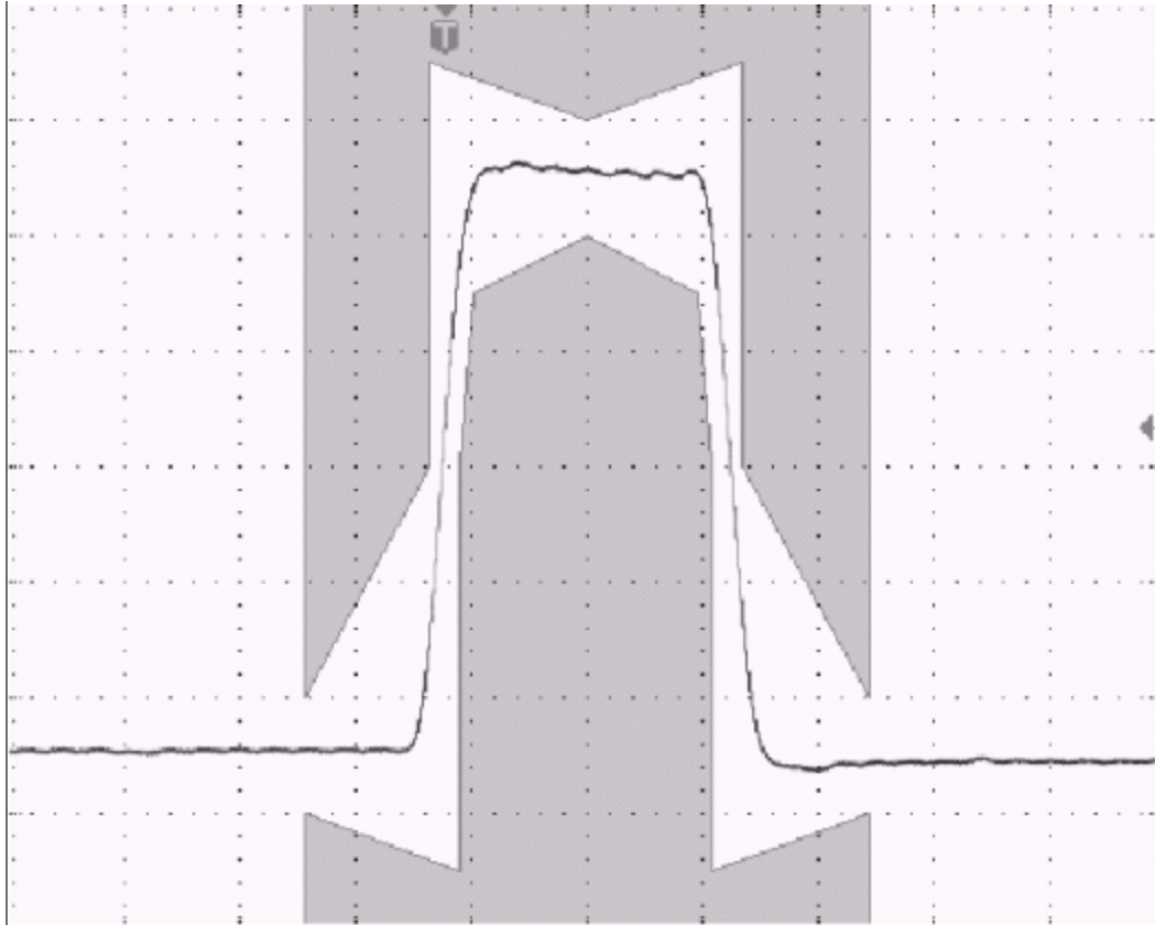
Figure 2. E1 Pulse (2.048 Mbits/s).
