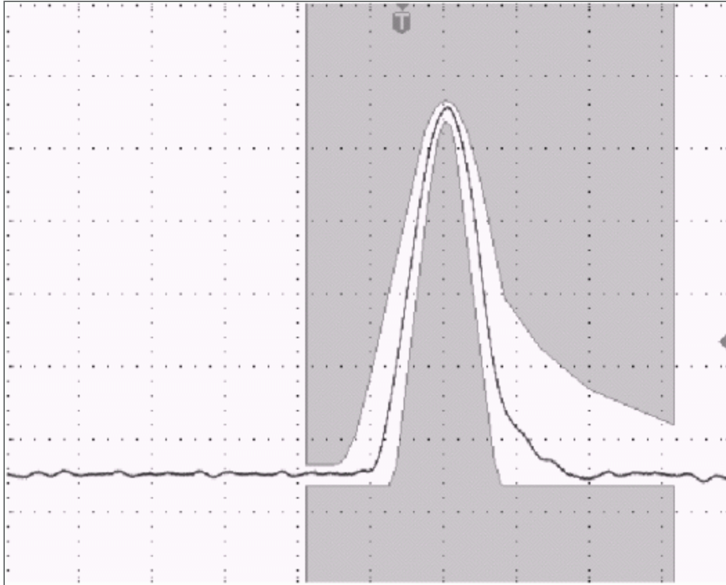
Figure 3. T3 Pulse (44.736 Mbits/s).
