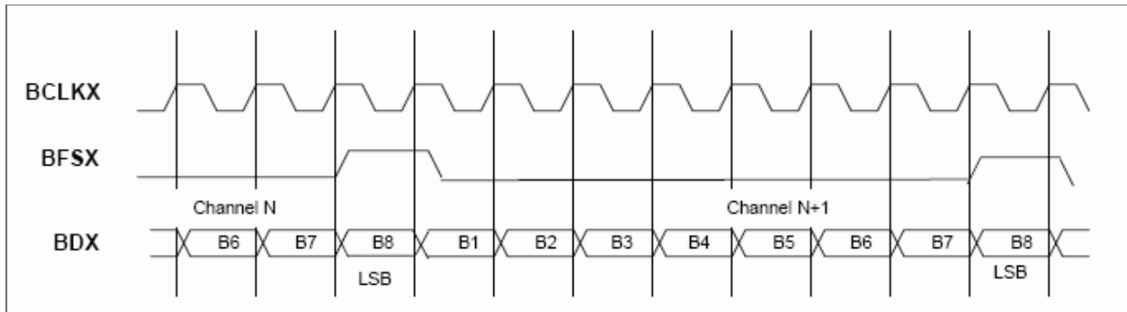
Figure 3. Burst Mode Transmit Timing (External Frame).
