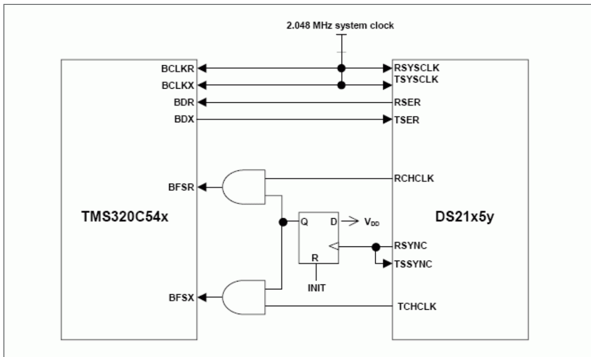
Figure 7. Block Diagram of the TMS320C54x and the DS21x5y Using a 2.048MHz System Clock Locked to the Network Clock.
