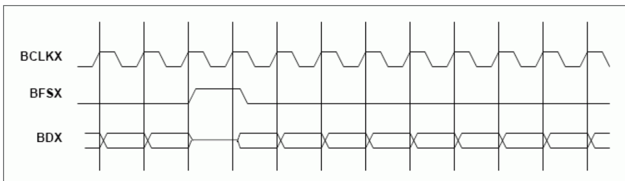
Figure 1. Continuous Mode Transmit Timing (External Frame).
