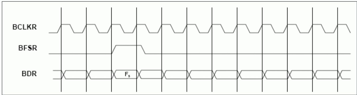
Figure 2. Continuous Mode Receive Timing (External Frame).
