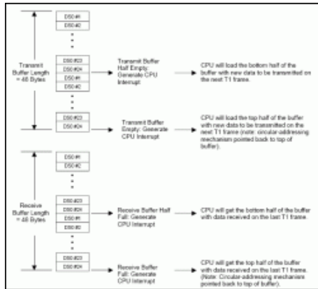
Figure 8. Autobuffering Unit Operation.
