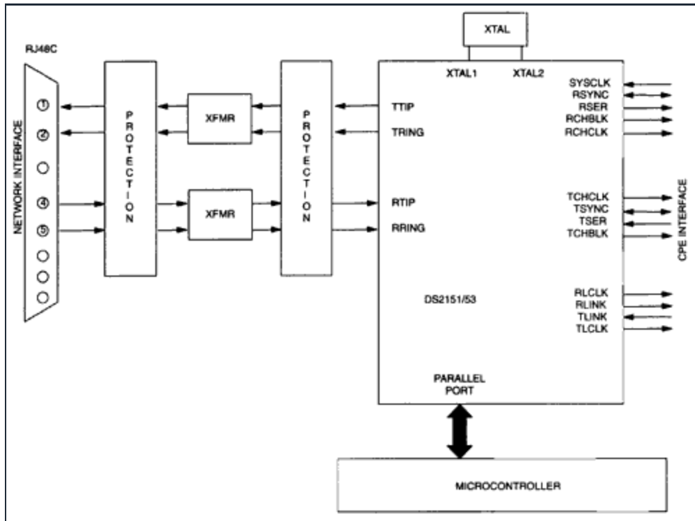
Figure 1. CSU Circuit.
