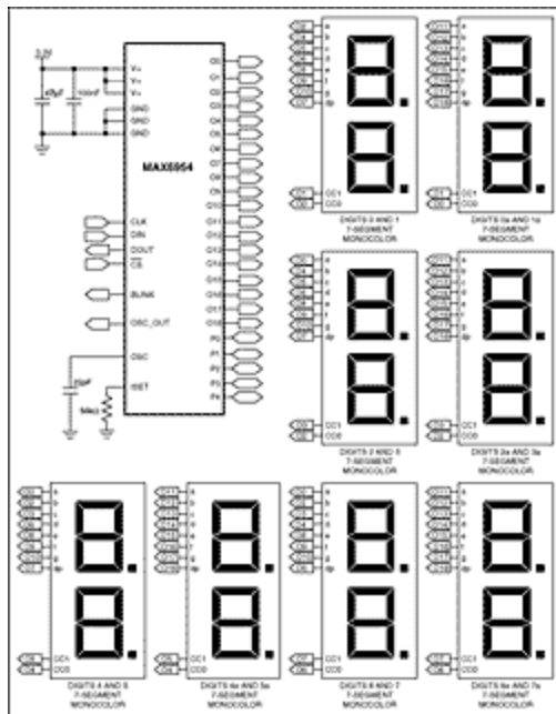
Figure 1. MAX6954 7-segment application circuit.
