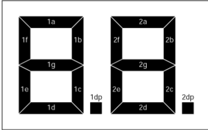
Figure 2. Segment labeling for 7-segment displays.
