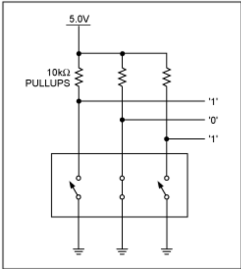
Figure 1. Mechanical DIP switch.
