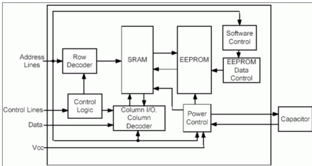
Figure 2. NOVRAMs.
