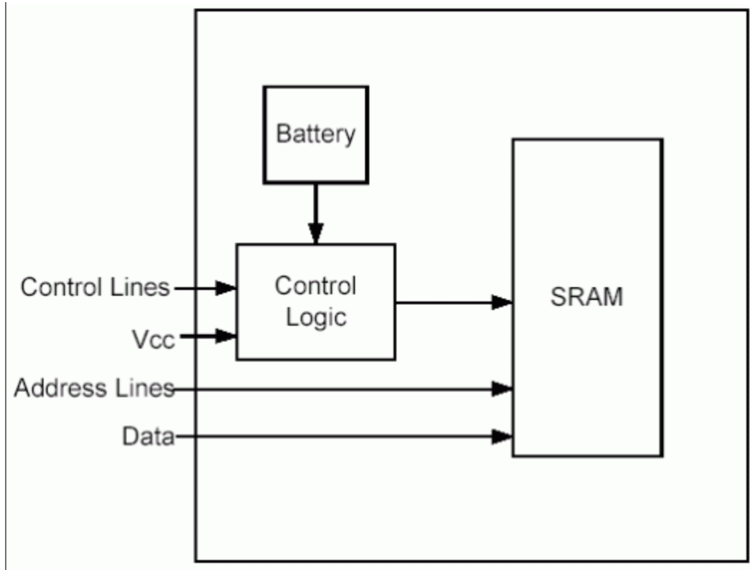
Figure 1. Battery-backed NVSRAM.
