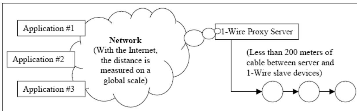
Figure 2. 1-Wire proxy example.
