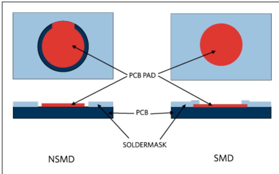
Figure 3. Illustration of NSMD and SMD land pad patterns.
