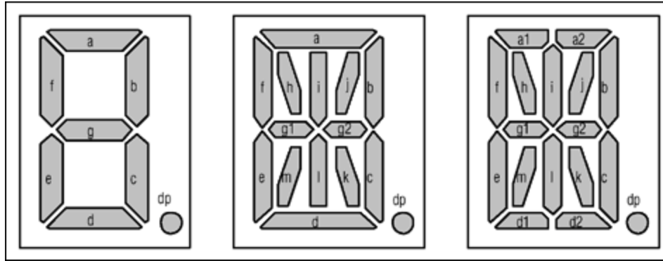
Figure 1. Segment labeling for 7-, 14-, and 16-segment displays.
