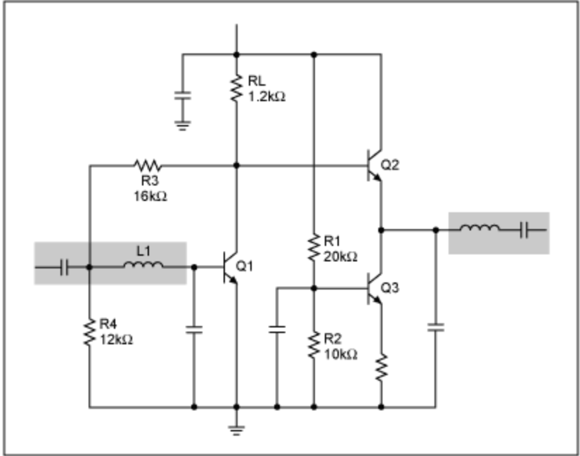
Figure 1. Simplified schematic of the LNA (gray area: off-chip matching).
